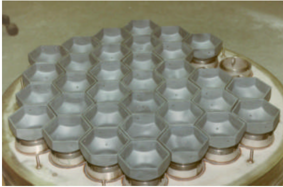
Fig. 5: HiTRec I stainless steel construction
