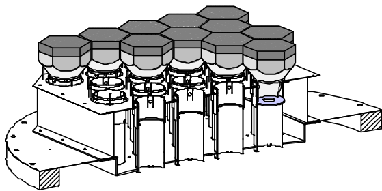
Fig. 9: Cut through the HiTRec II receiver design
