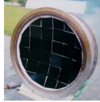
Fig. 3: CorRec Receiver
