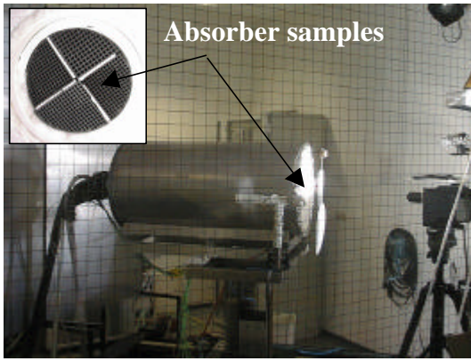
Fig. 13: Cycle test for heliotech absorber materials in the solar furnace at DLR
