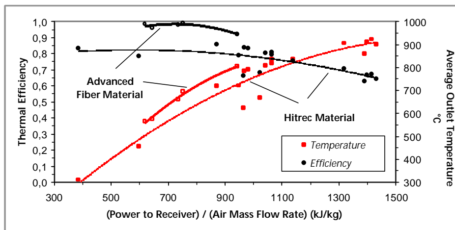
Fig. 16: Efficiency Test Results from an Advanced Absorber Material compared to the HiTRec Material
