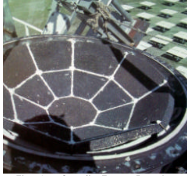
Fig. 2: Sandia Foam Receiver
