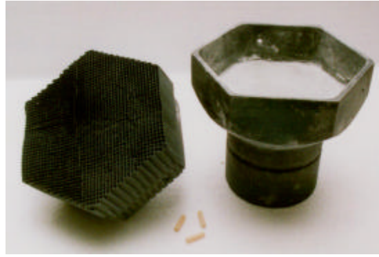
Fig. 6: HiTRec I absorber module, monolith and cup
