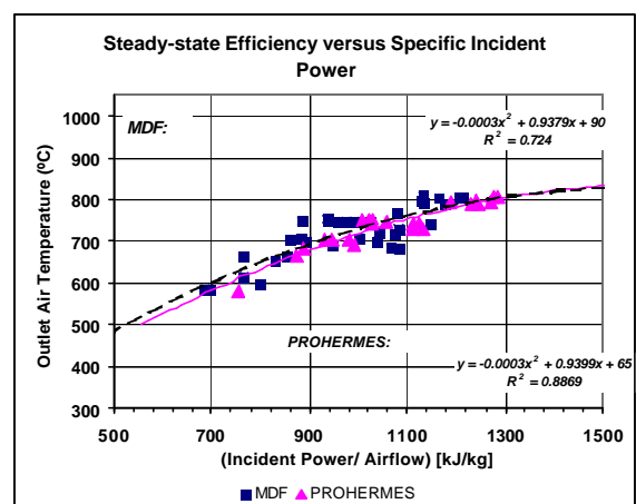
Fig. 12: Average outlet temperature versus specific incident power
