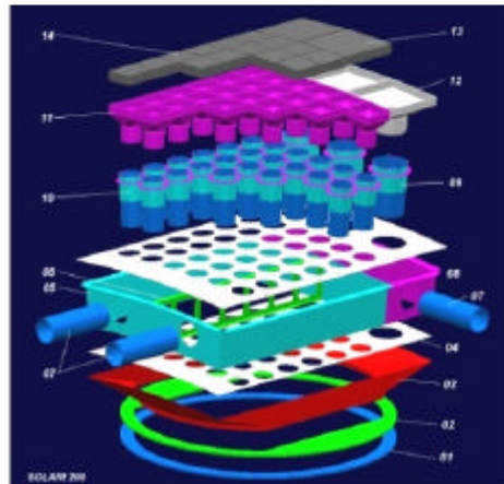
Fig. 15: Solair 200 receiver design
