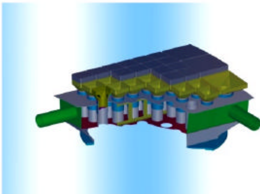
Fig. 15: Solair 200 receiver design
